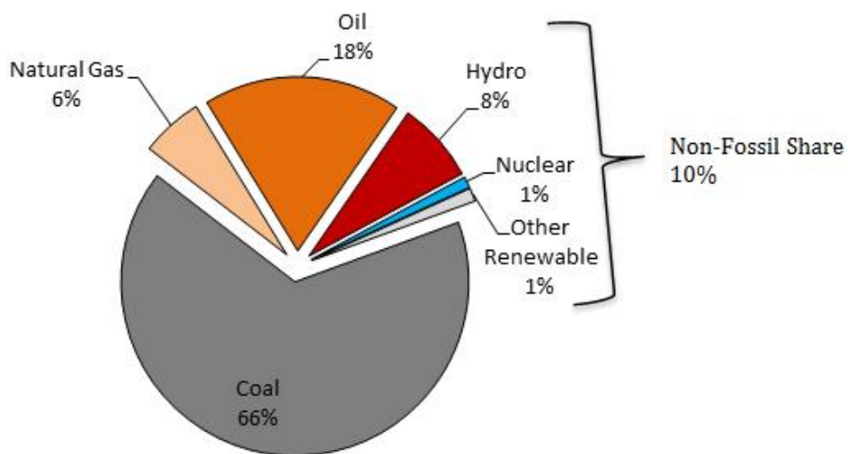
Total energy consumption in China by type, 2013
