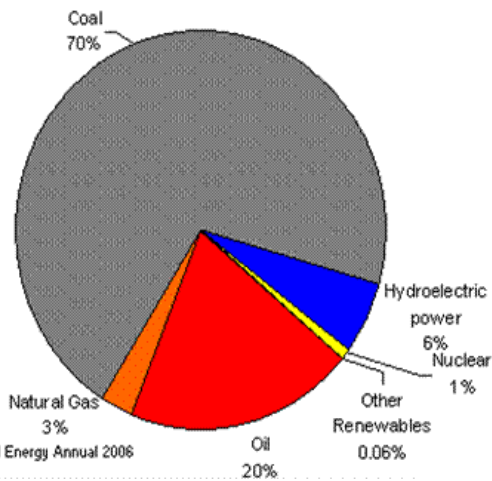
Total Energy Consumption in China, by Type (2006)
